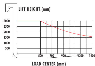
CAPACITY CHART
